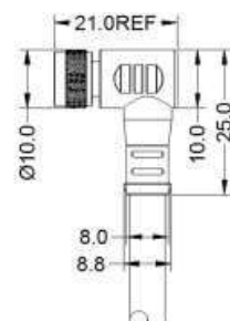
A Code 8 pins
