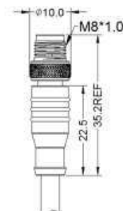
A Code 8 pins
