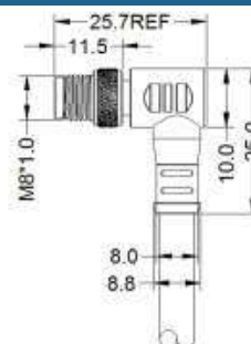
A Code 8 pins
